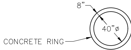
SECTION B-B (CONCRETE THROAT) (OPTION A)
