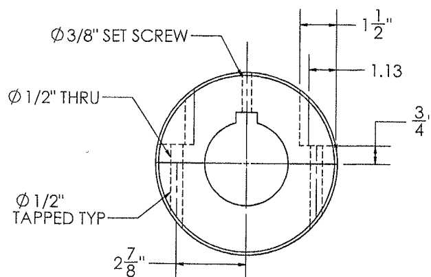
HUB DETAIL
