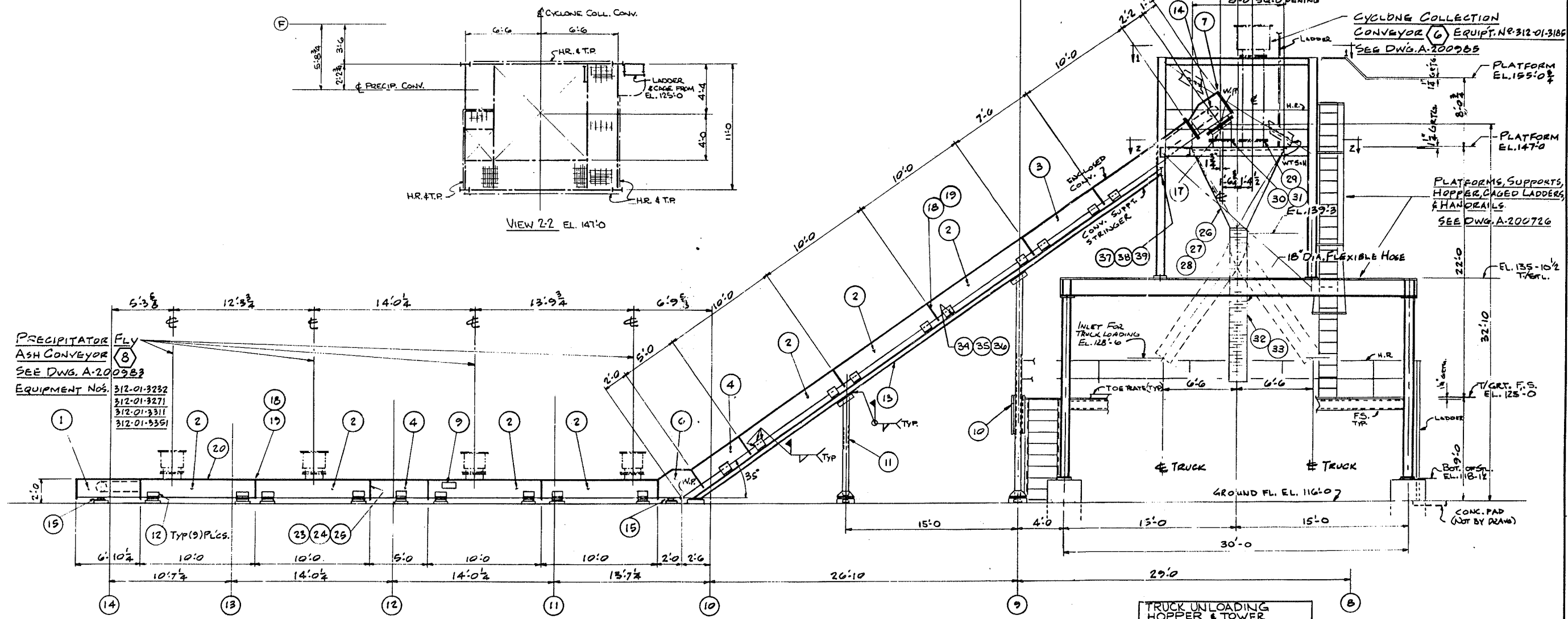
ELEVATION G-G FROM DWG. A-200990 (SHT. 2) (6"x18") 7 PRECIPITATOR TRANSFER CONVEYOR EQUIPMENT NO. 312-01-3355
